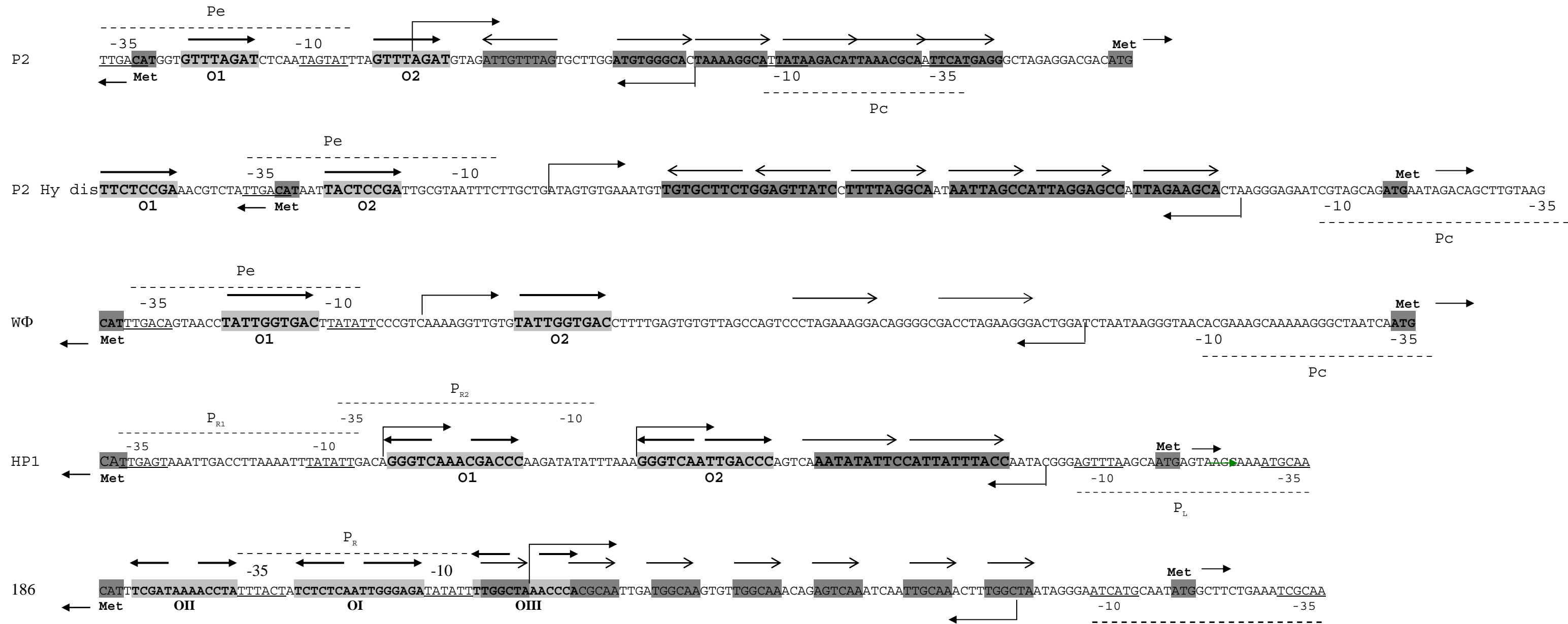
Fig. 25-10. The nucleotide sequences of the promoter-operator regions of P2 and some P2-like phages. The -10 and -35 regions are underlined, and the start of the transcripts are indicated with bend arrows. The operators for the immunity repressors are indicated by light gray shadings, and those of the Cox/Apl repressors in dark gray shadings. The arrows above the shaded operators indicate the orientation of the respective recognition sequence for each protein. The start codons of the genes are indicated.
